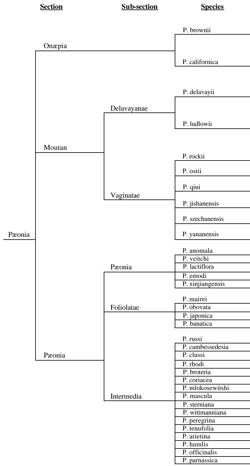
Fig. 1. Phylogenetic tree of Genus Pæonia based on the recent studies of Sang, Hong † et al. and Hong * et al.
